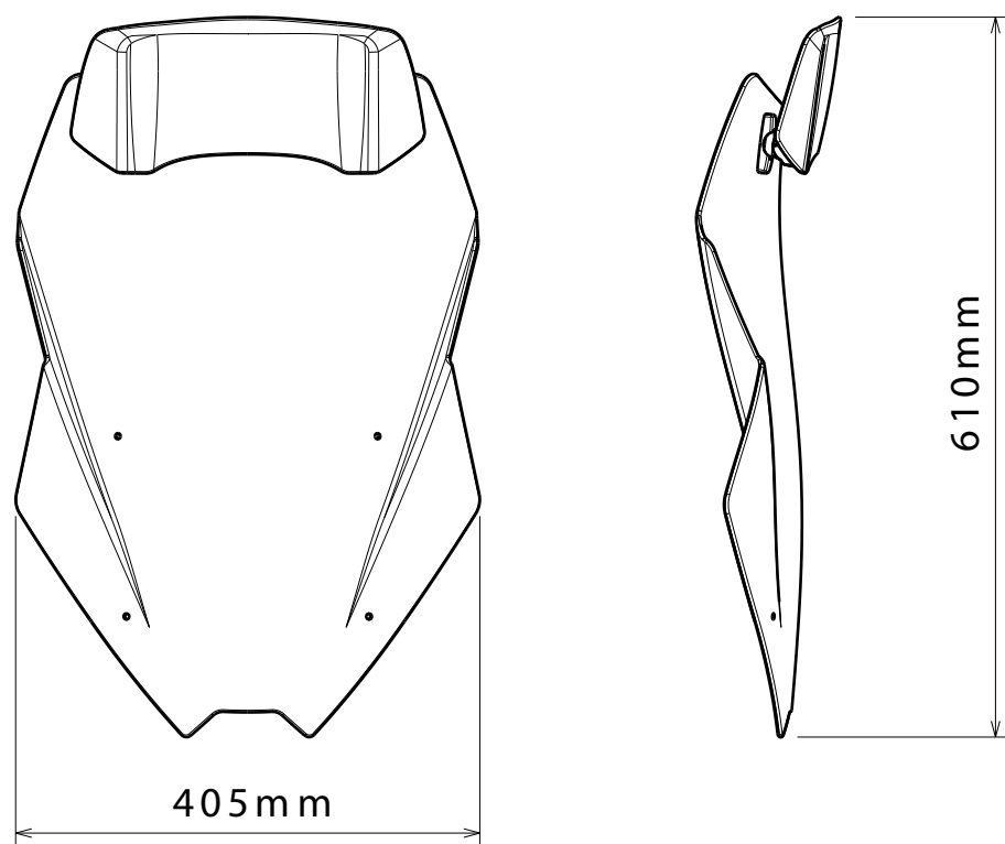
TOURING SCREEN WITH VISOR AT HIGHER POSITION
