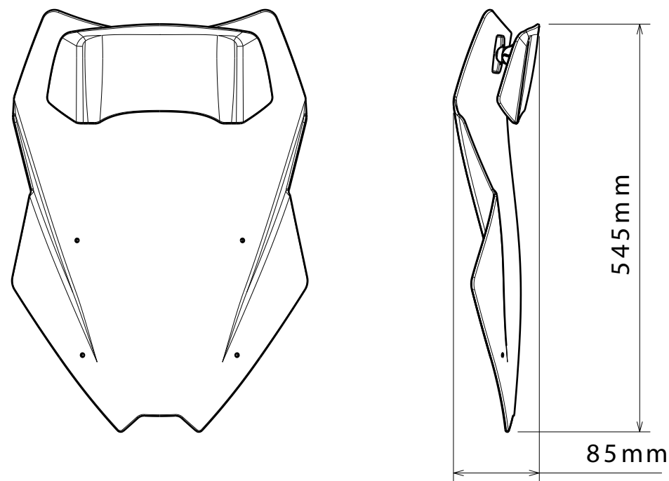
TOURING SCREEN WITH VISOR AT LOWER POSITION
